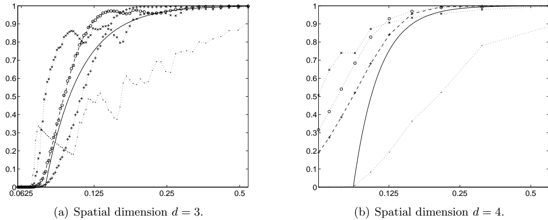
Figure 3.1: Minimal eigenvalue of the interpolation matrix \mathbf{Y}\hat{\mathbf{W}}\mathbf{Y}^H with respect to the separation distance q\lambda for a fixed polynomial degree N = 50 . The order of the B-spline kernel and hence the localization order is \beta = 1 ( \cdot ), \beta = 2 ( \times ), \beta = 3 ( \circ ), and \beta = 4 ( + ). Moreover, we plotted the estimate 1 - (\frac{C_d}{(N+1)q})^d (solid) and additionally the minimal eigenvalue for \beta = d (dashed).
