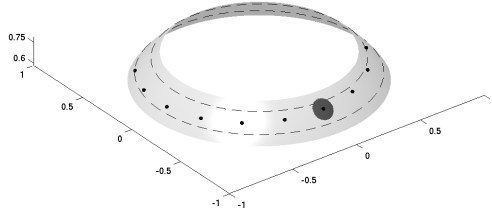
Figure 2.1: The set S_{\mathcal{X},q,m} , the ring S_{q,m} (dashed), the larger ring \tilde{S}_{q,m} , and a spherical cap of colatitude q/2 centered at one node for generalized spiral nodes, cf. [26], on the sphere \mathbb{S}^2 .
